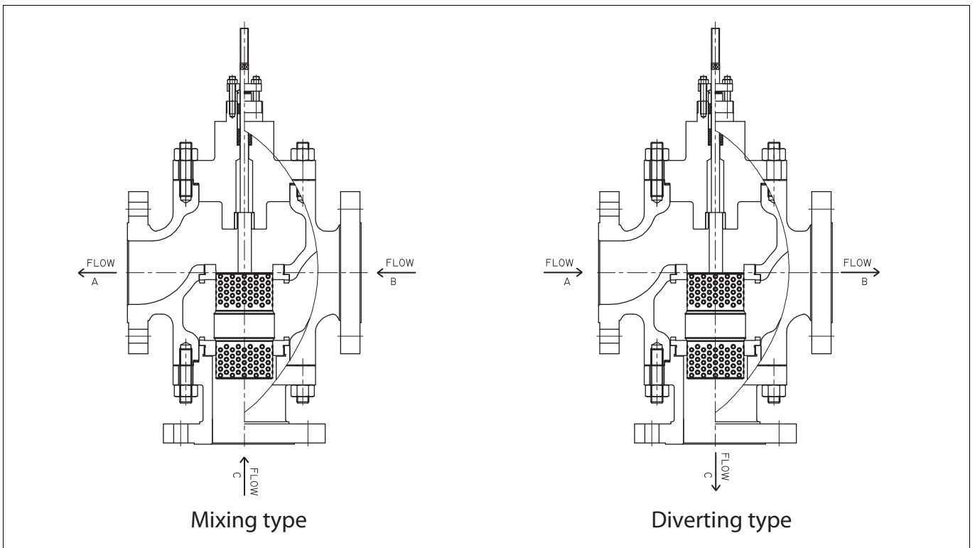
Fig. 1 Construction of the Neles GW series 3-way Valve
