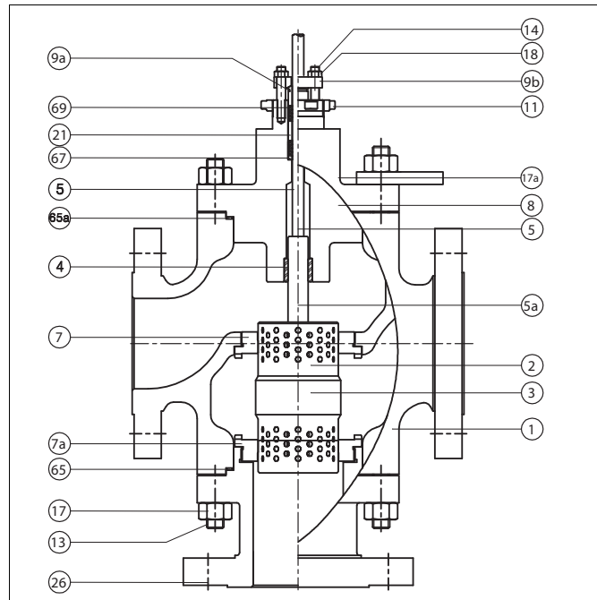
Fig. 9 Conventional Cylindrical Plug Trim
