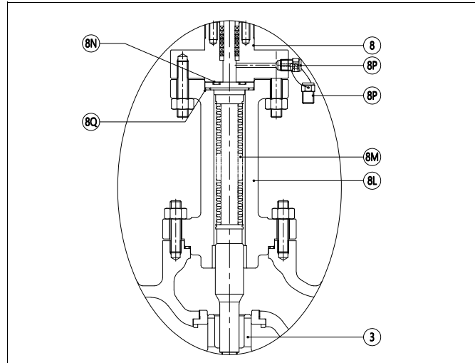
Fig. 6 Bellows seal construction
