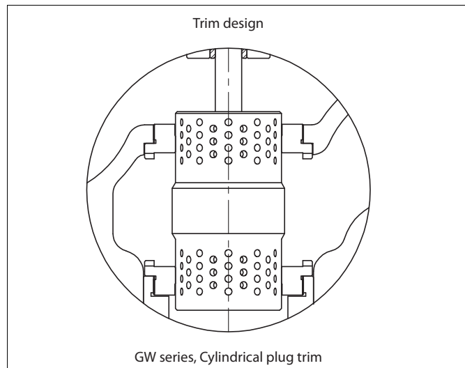
Fig. 10 Trim design
